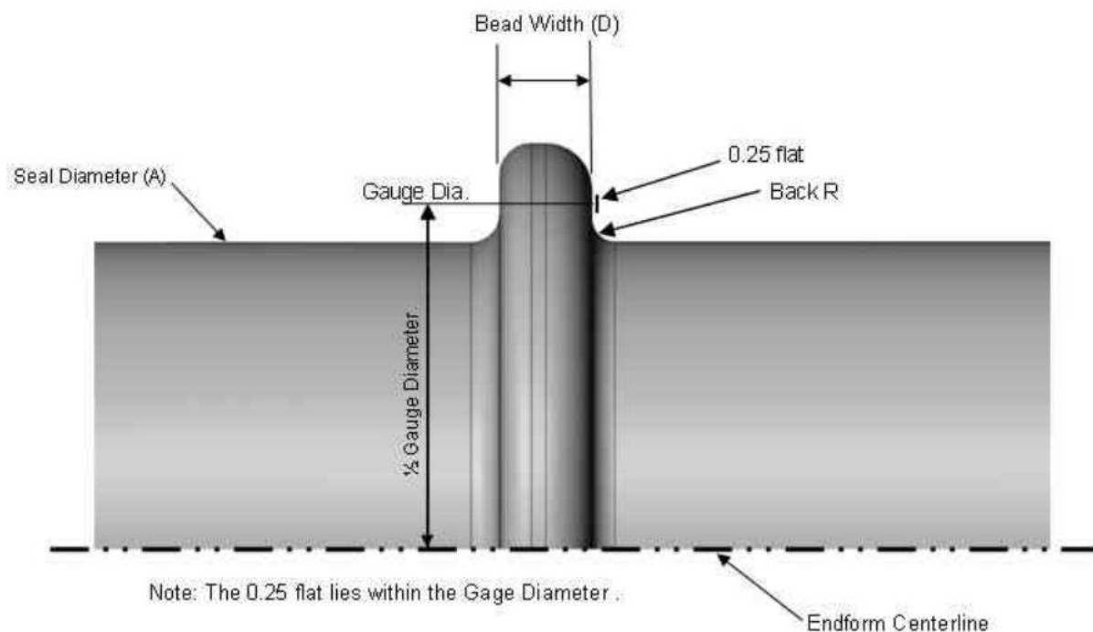
FIGURE A1 - BEAD WIDTH MEASUREMENT
