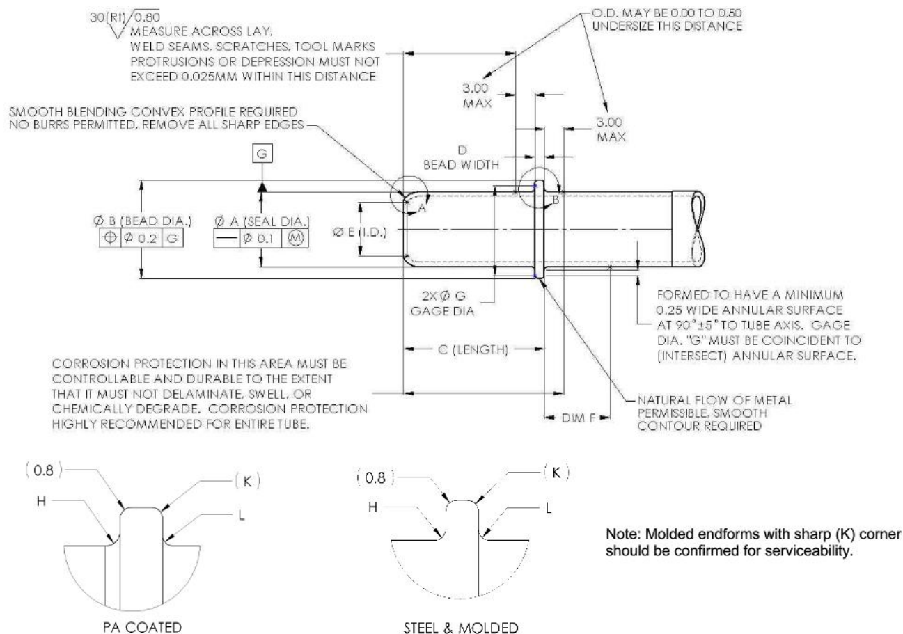
FIGURE 2 - MATING TUBE END FORM
